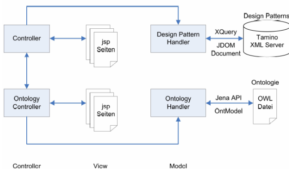
Fig. 4: Model View Controller Architecture
